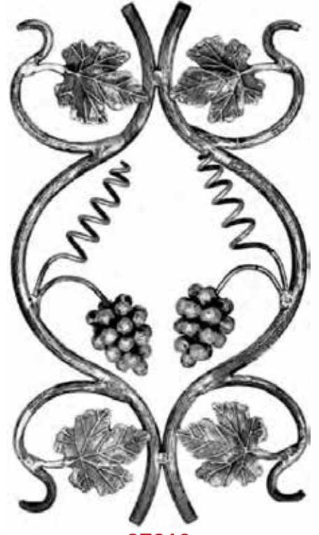
27310 Ø14 mm 3,710 kg 285x500
